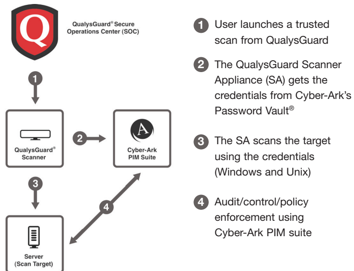
Figure 1: Workflow of the integration between QualysGuard and Cyber-Ark PIM Suite
